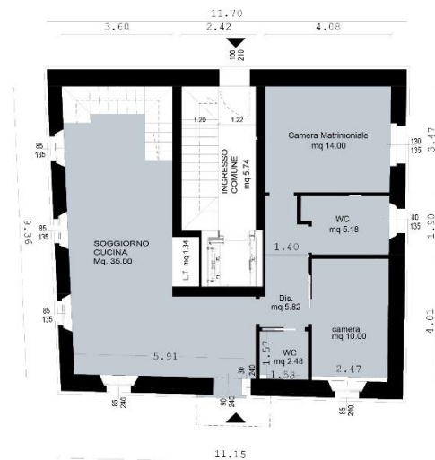
PIANO TERRA
